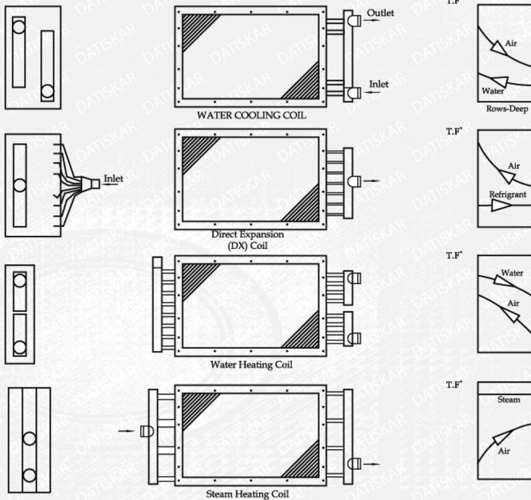
COIL TYPES & TEMPERATURE PROFILES THROUGH THE COILS
